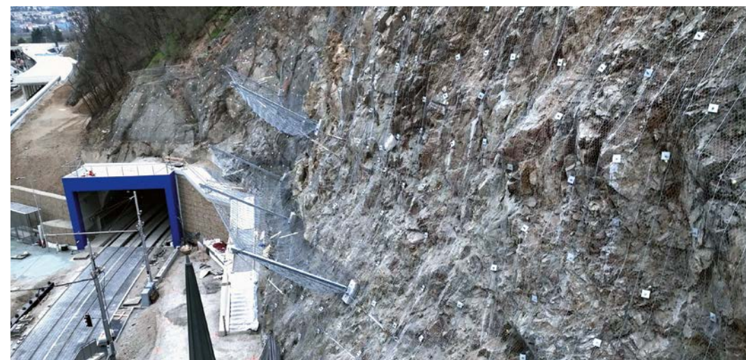
Dynamic Barriers, Brno, Czech Republic
