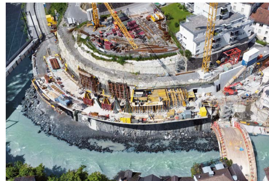
Flood Protection, Kapfchlucht, Austria
