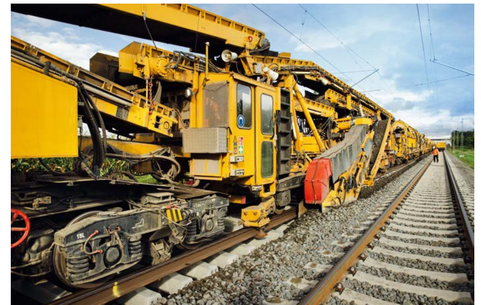
RU 800 S Track Renewal Train
